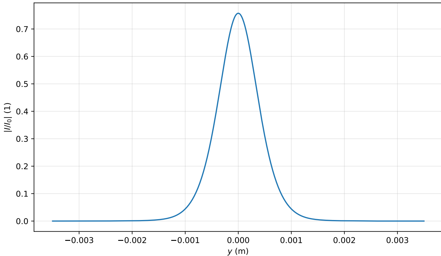
Intensity profile I(x=0, y, z=3.344)/I_0 , P_{in}=0.7P_{cr} , artificial time
